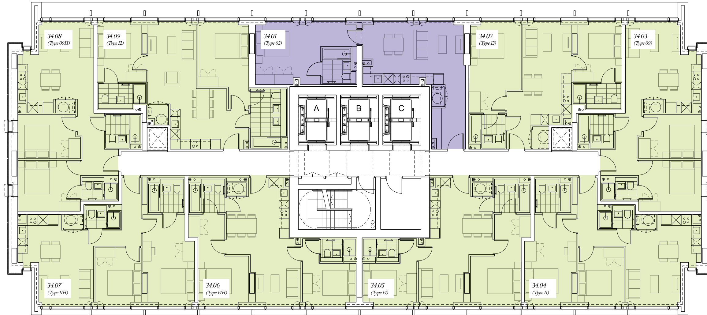
1 Bed Apartment 34.01 - (Type 03)
