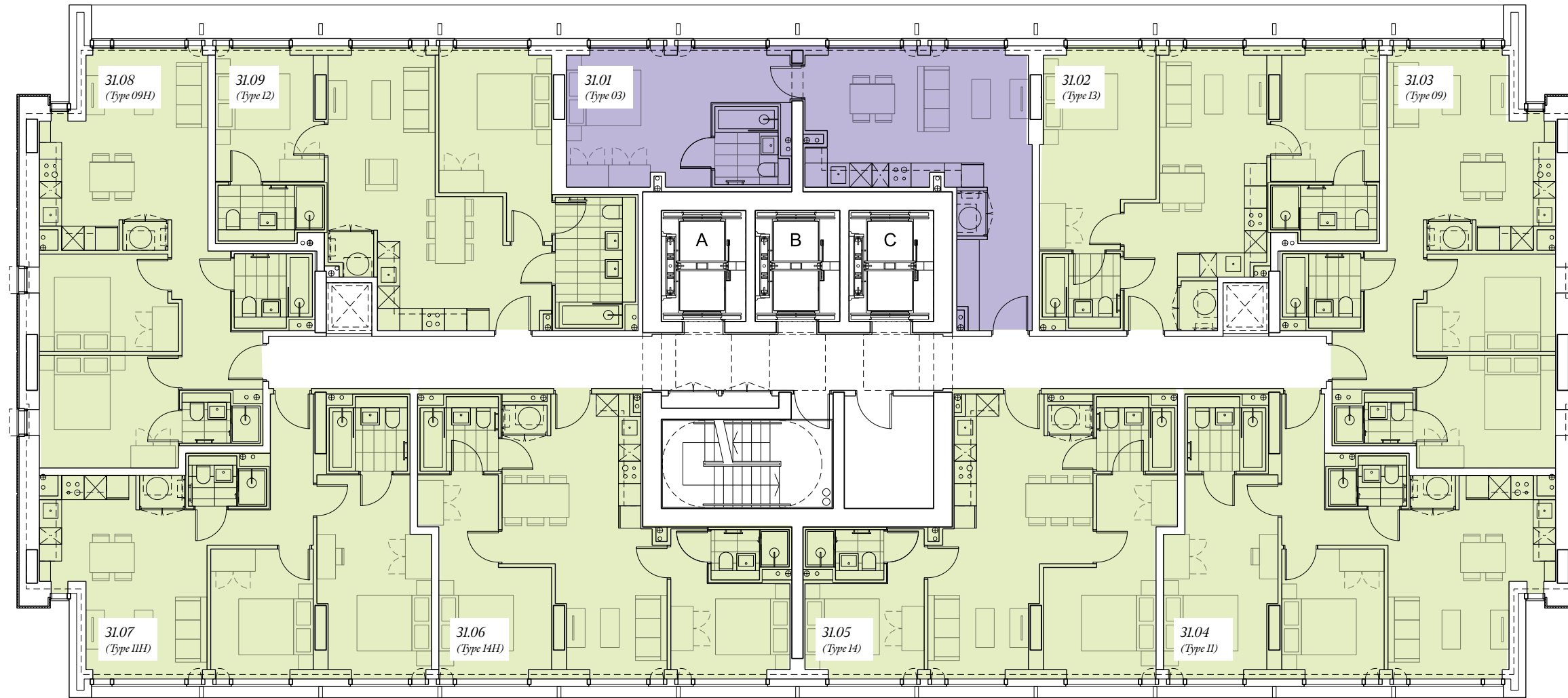
1 Bed Apartment 31.01 - (Type 03)
