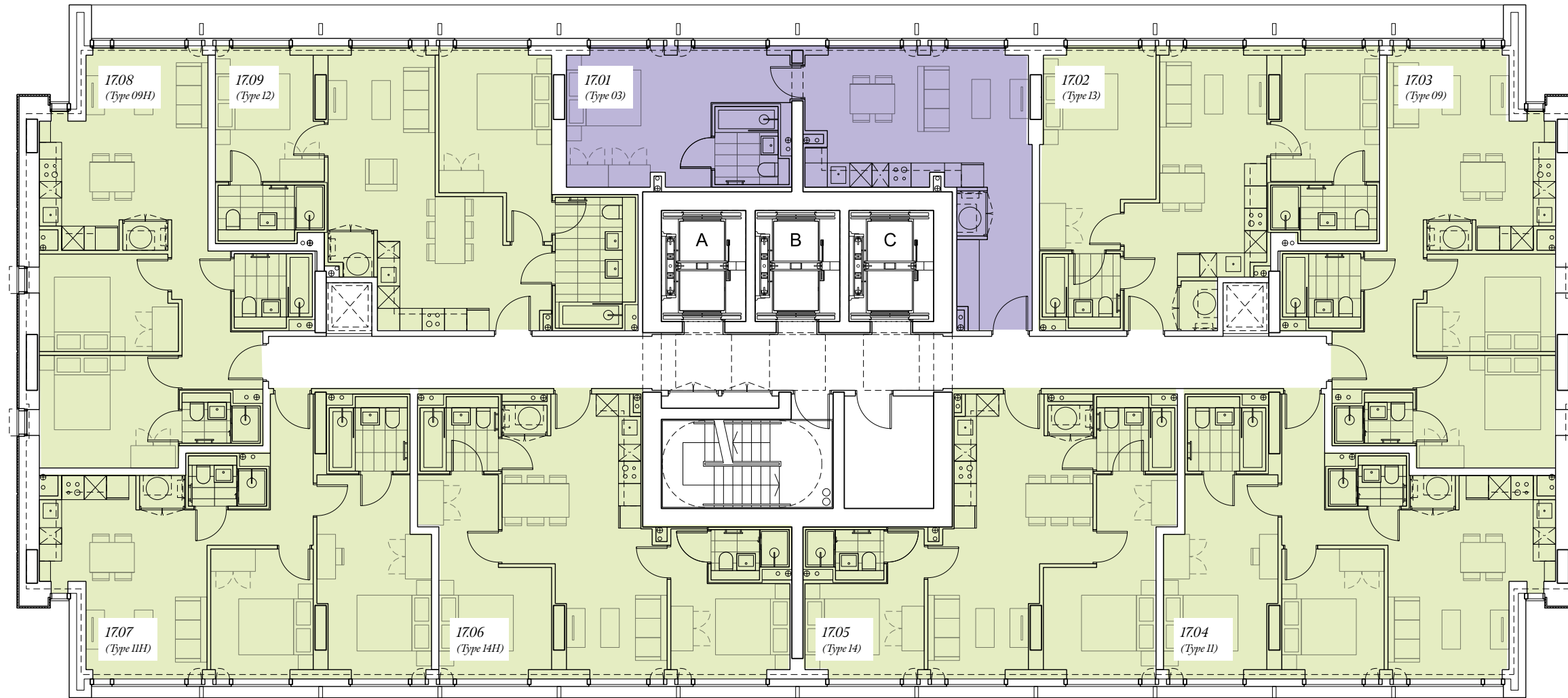
1 Bed Apartment 1701 - (Type 03)
